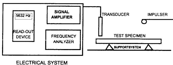
FIG. 1 Block Diagram of Typical Test Apparatus
