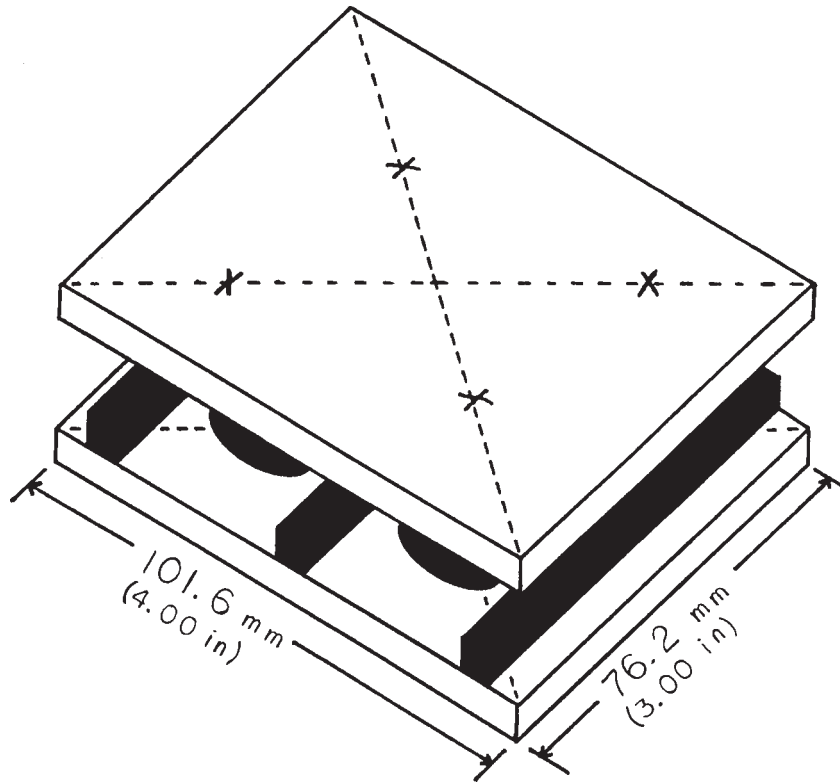
FIG. 2 Steel Spacers
