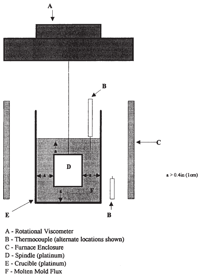
FIG. 1 Typical Crucible/Spindle Configuration
