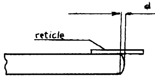
FIG. 5 Depth Measurement of Beveled Region
