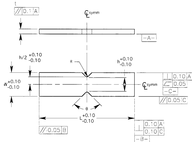
FIG. 5 Schematic of the Iosipescu Specimen
