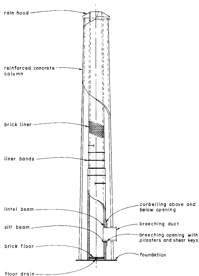
FIG. 4 General Arrangement
