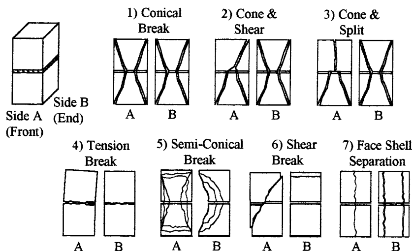
FIG. 4 Sketches of Mode of Failure
