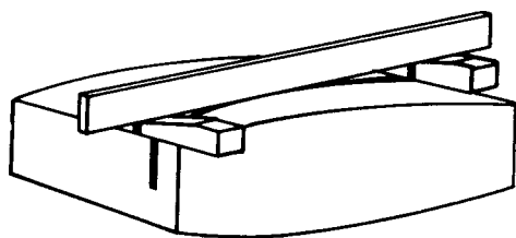
FIG. 3 Method of Measuring Warpage of a Convex Surface
