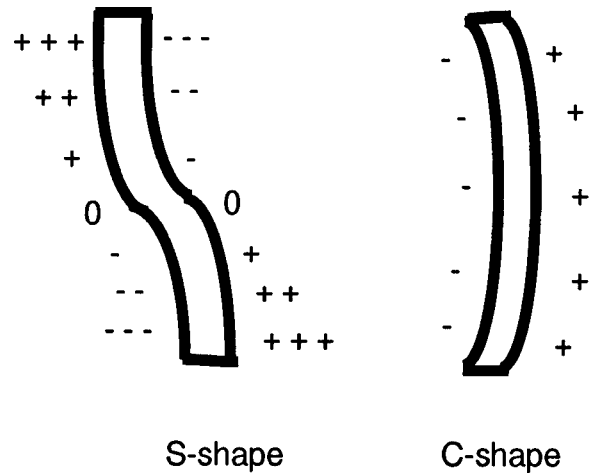
FIG. X1.2 S-Shape and C-Shape Bending of Tensile Specimen
