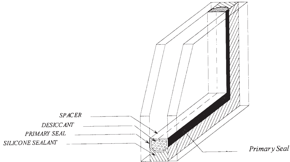
FIG. 1 Cutaway Section of IG Unit Edge Seal
