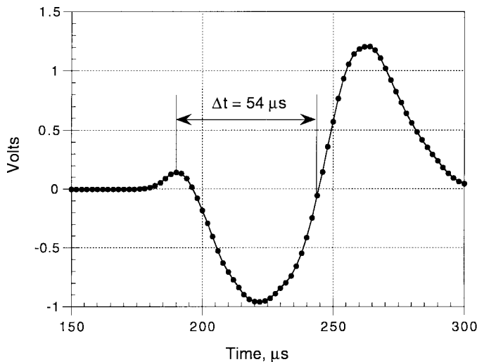
FIG. 1 Expanded View of Surface-Wave Portion of Waveform Showing the Width of the Surface Wave Signal as an Approximation of the Contact Time of the Impact
