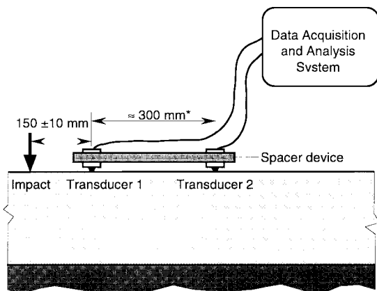
FIG. 2 Schematic of Testing Configuration for Procedure A
