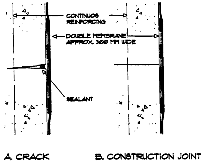
FIG. 4 Reinforced Joints
