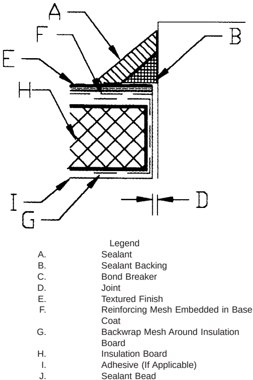
FIG. 9 Sealant Fillet Joint Seal With Triangular Sealant Backing
