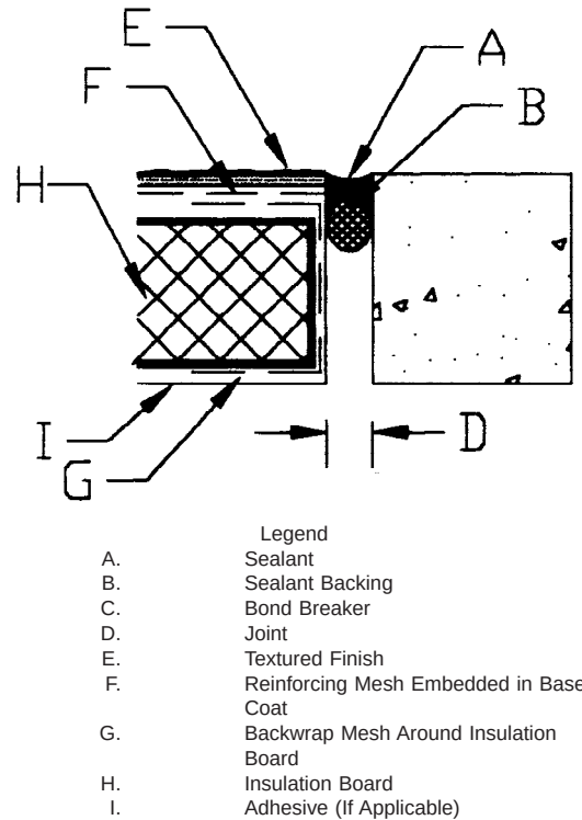
FIG. 2 Sealant Butt Joint Seal (EIFS to Dissimilar Substrates)
