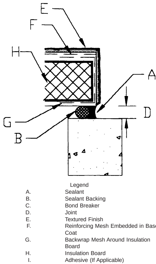
FIG. 11 Sealant Lap Joint Seal
