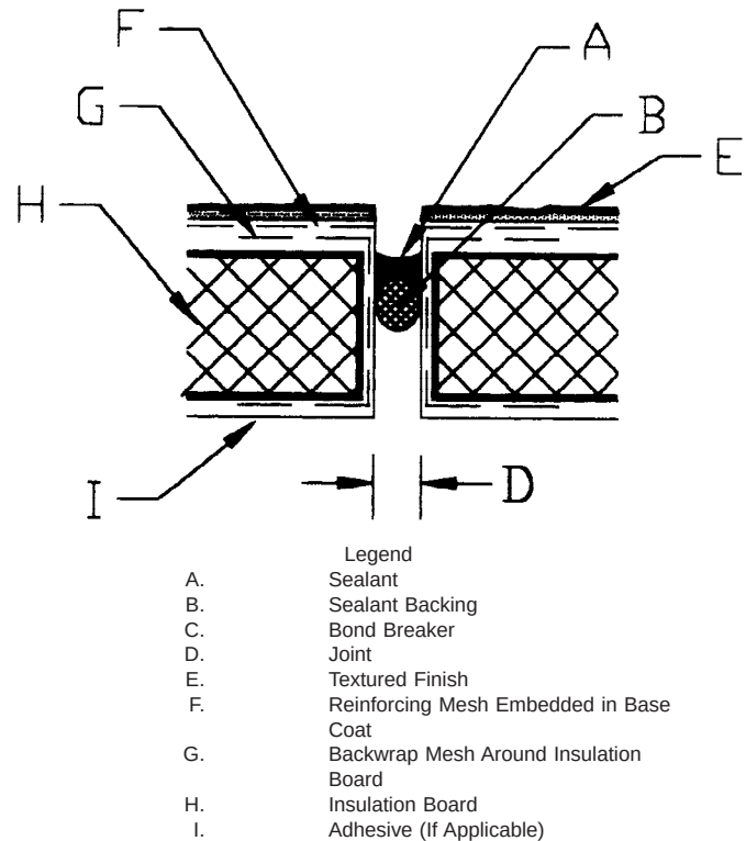
FIG. 3 Recessed Sealant Butt Joint Seal (EIFS to EIFS)
