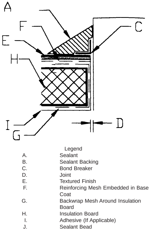
FIG. 8 Sealant Fillet Joint Seal With Bond Breaker
