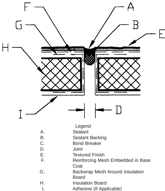
FIG. 1 Sealant Butt Joint Seal (EIFS to EIFS)
