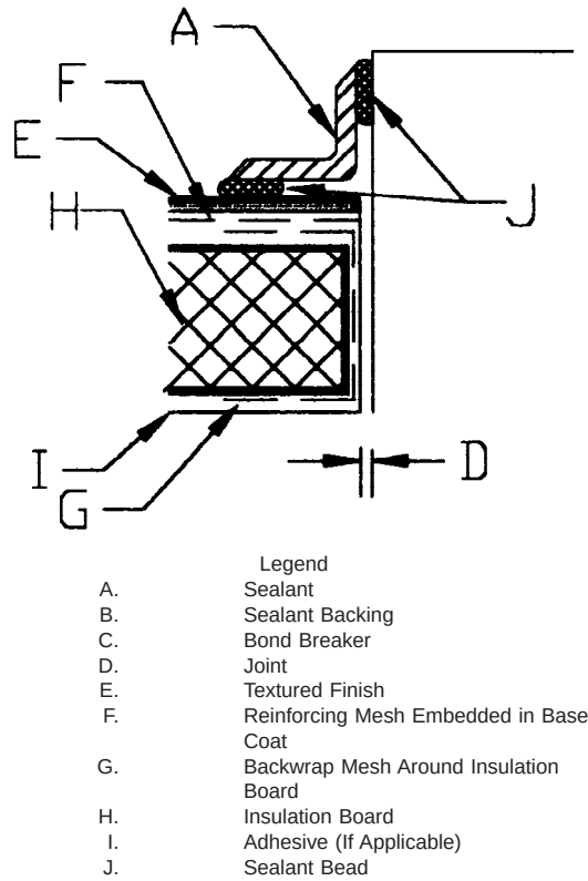
FIG. 10 Sealant Fillet Joint Seal Using Precured Sealant
