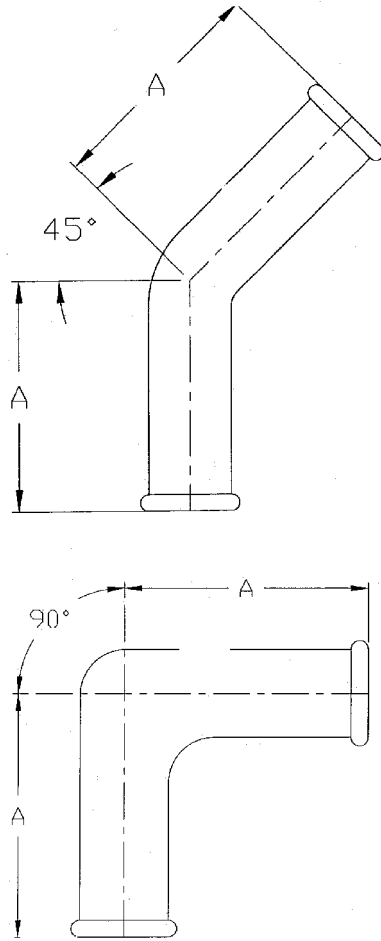
Dimensions A
