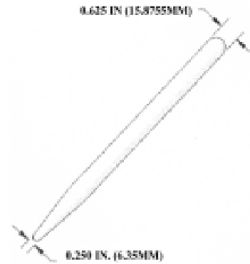
FIG. 1 Probing Tool
