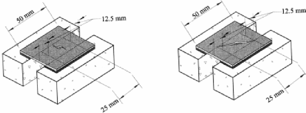
FIG. 5 Partial Tear
