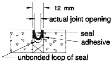
FIG. 3 U-joint Configuration
