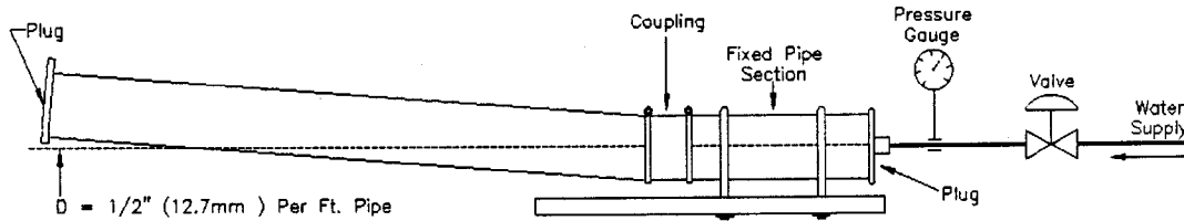
FIG. 1 Deflection Test
