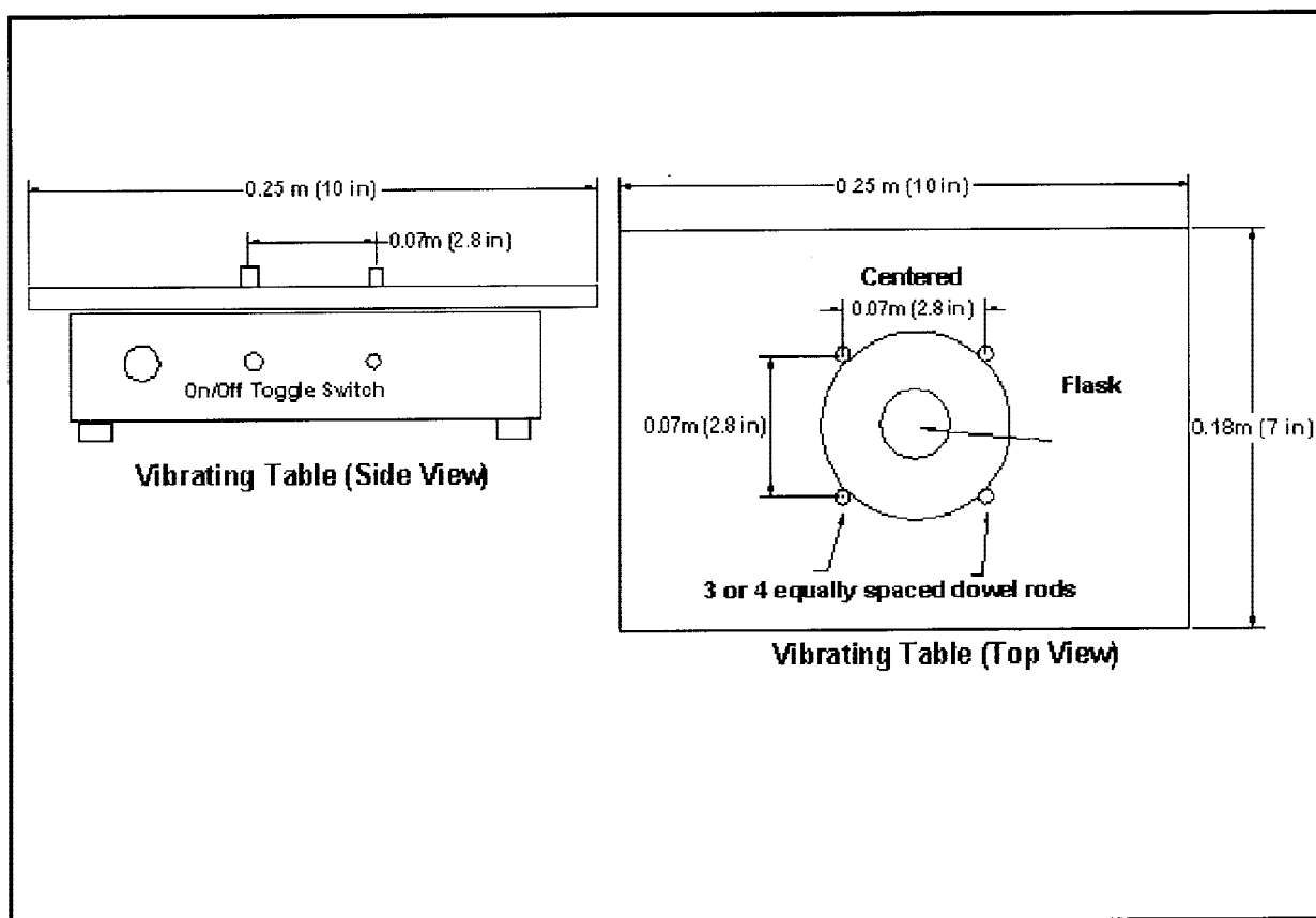
FIG. 1 Vibrating Table
