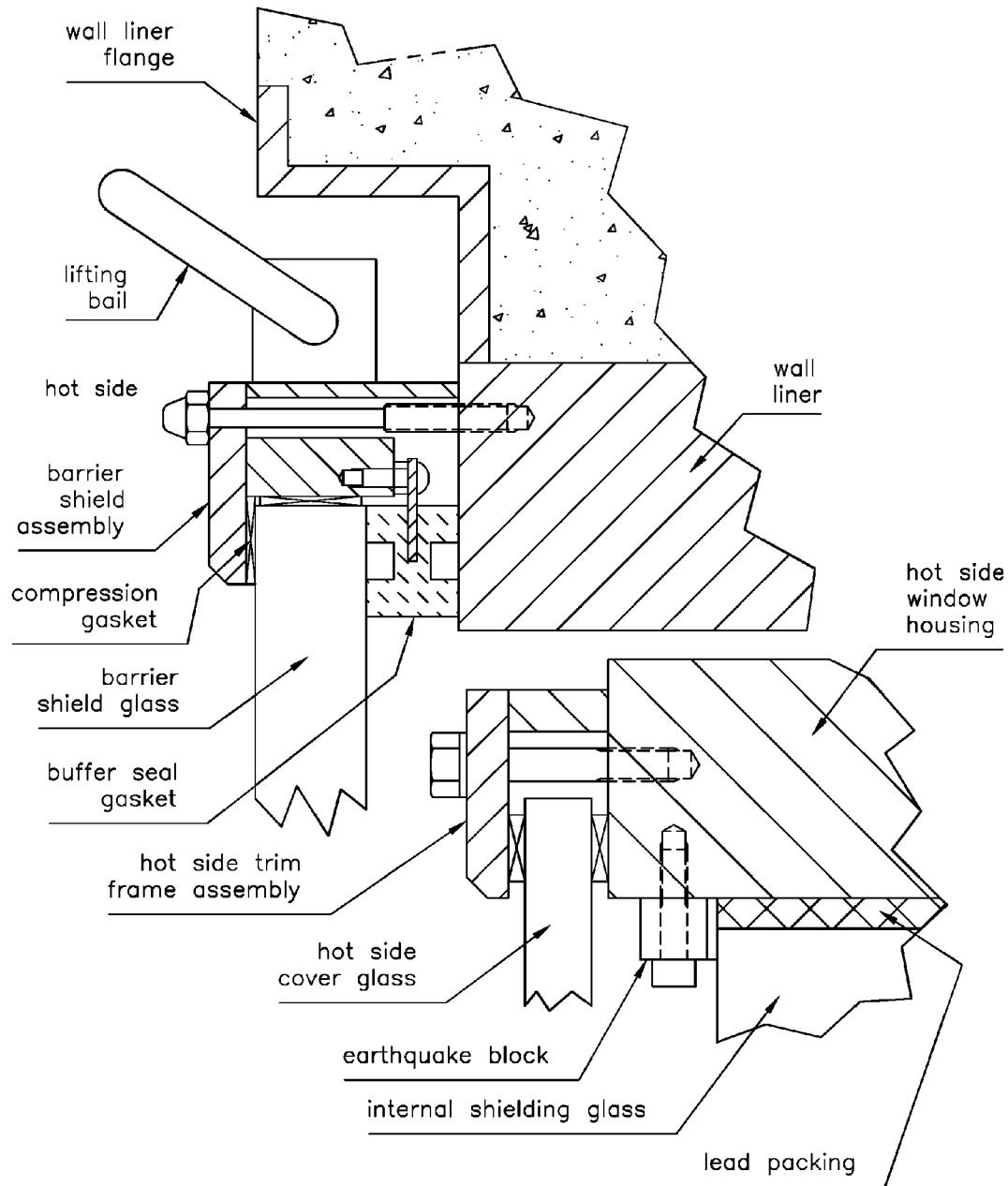
BARRIER SHIELD & HOT SIDE COVER GLASS det A
