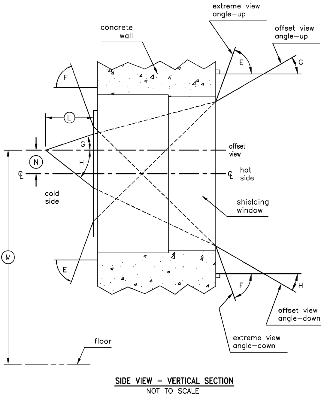
Annex A3 Figure 5 Typical Shield Window - Offset Viewing Angles in Vertical Section
