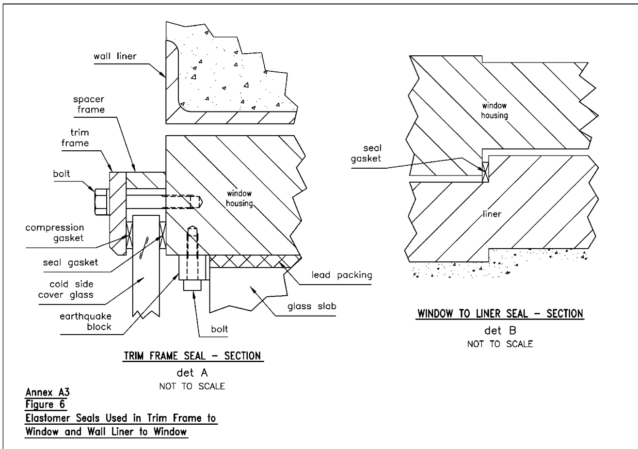
FIG. A3.6 Elastomer Seals Used in Trim Frame to Window and Wall Liner to Window
