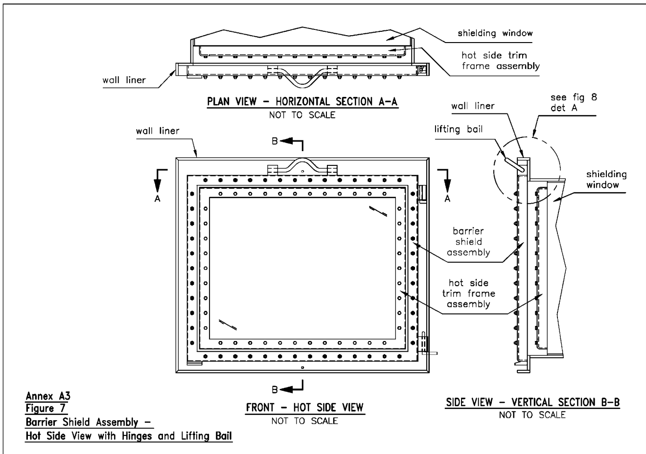
FIG. A3.7 Barrier Shield Assembly—Hot Side View with Hinges and Lifting Bail
