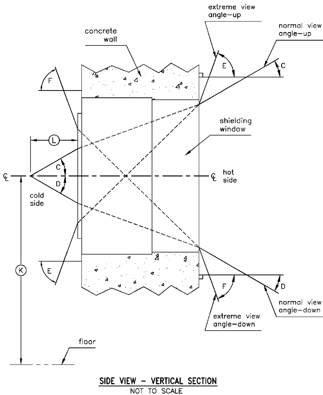
Annex A3 Figure 4 Typical Shield Window - Centerline Viewing Angles in Vertical Section
