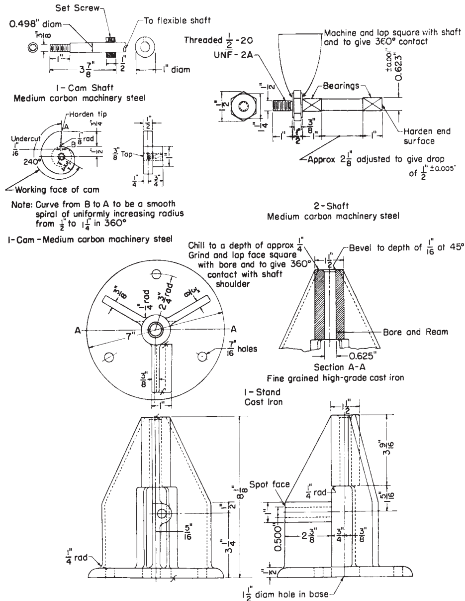
FIG. 1 Flow Table and Accessory Apparatus (Partial) (In./Lb)
