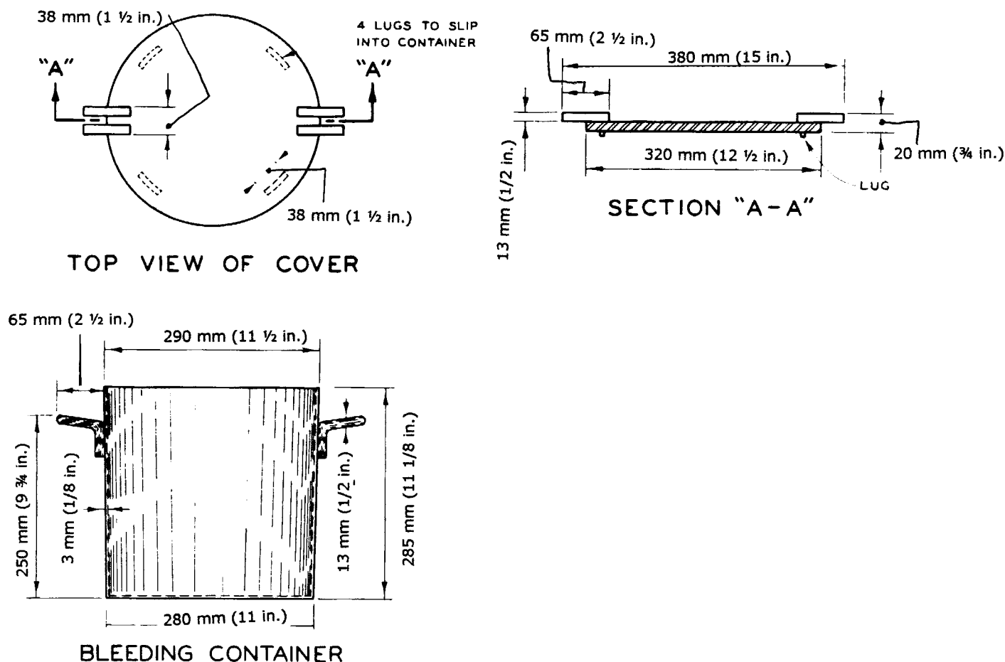
FIG. 3 Container and Cover
