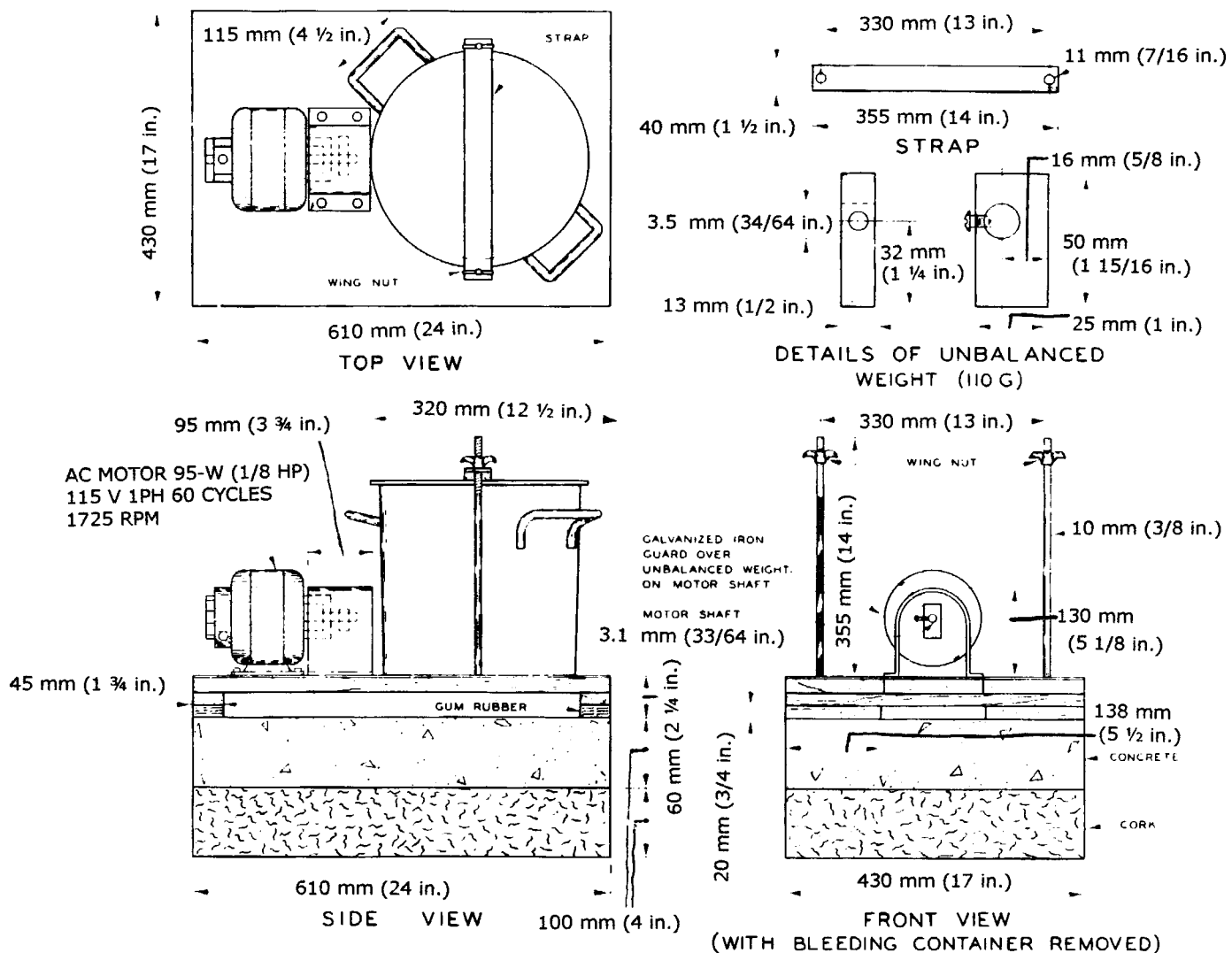
FIG. 2 Detail of Vibrating Platform Apparatus
