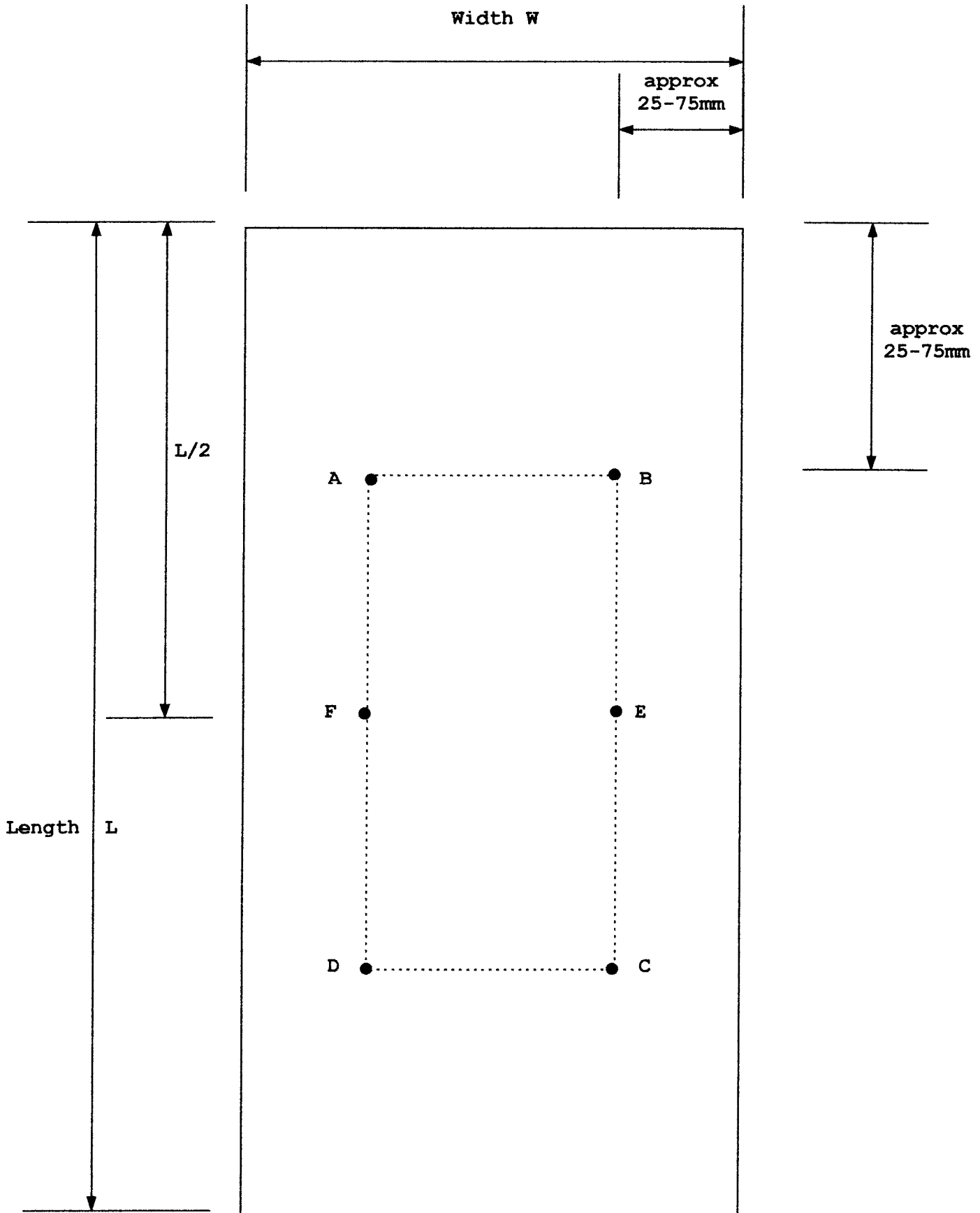
FIG. 1 Specimen Measurement
