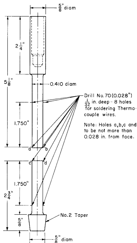
FIG. 2 Detail of Thermodes for 0.410-in. (10.41-mm) Diameter Specimen
