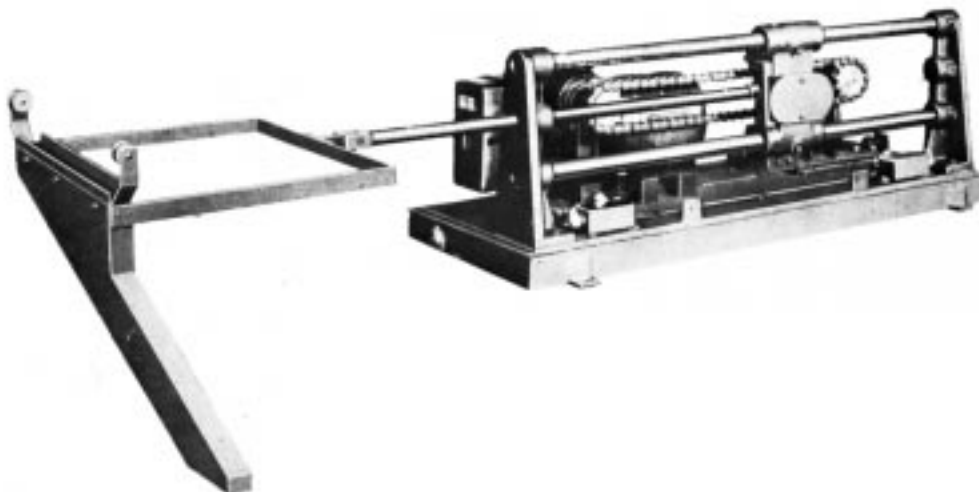
FIG. X2.4 Automatic Sampler
