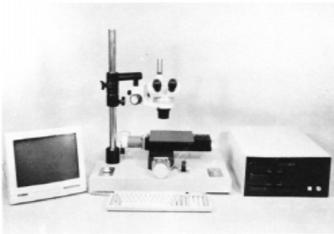
FIG. 3 Photograph of a Computerized Linear-Traversal/Point-Count Device Meeting the Requirements of This Test Method
