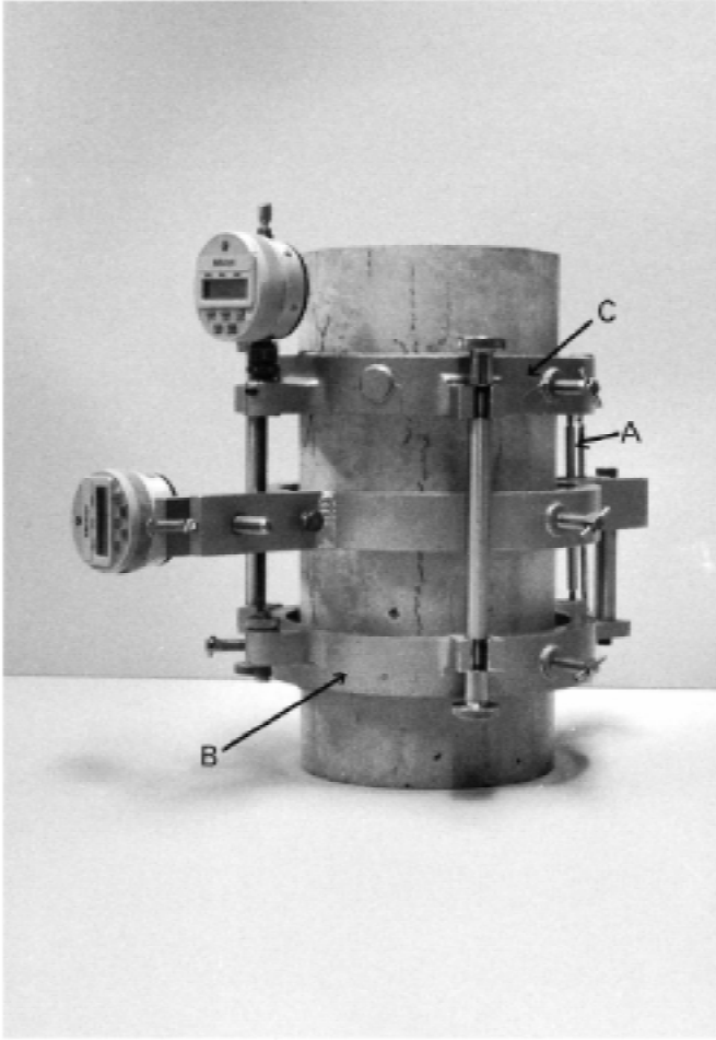
FIG. 1 Sutable Compressometer
