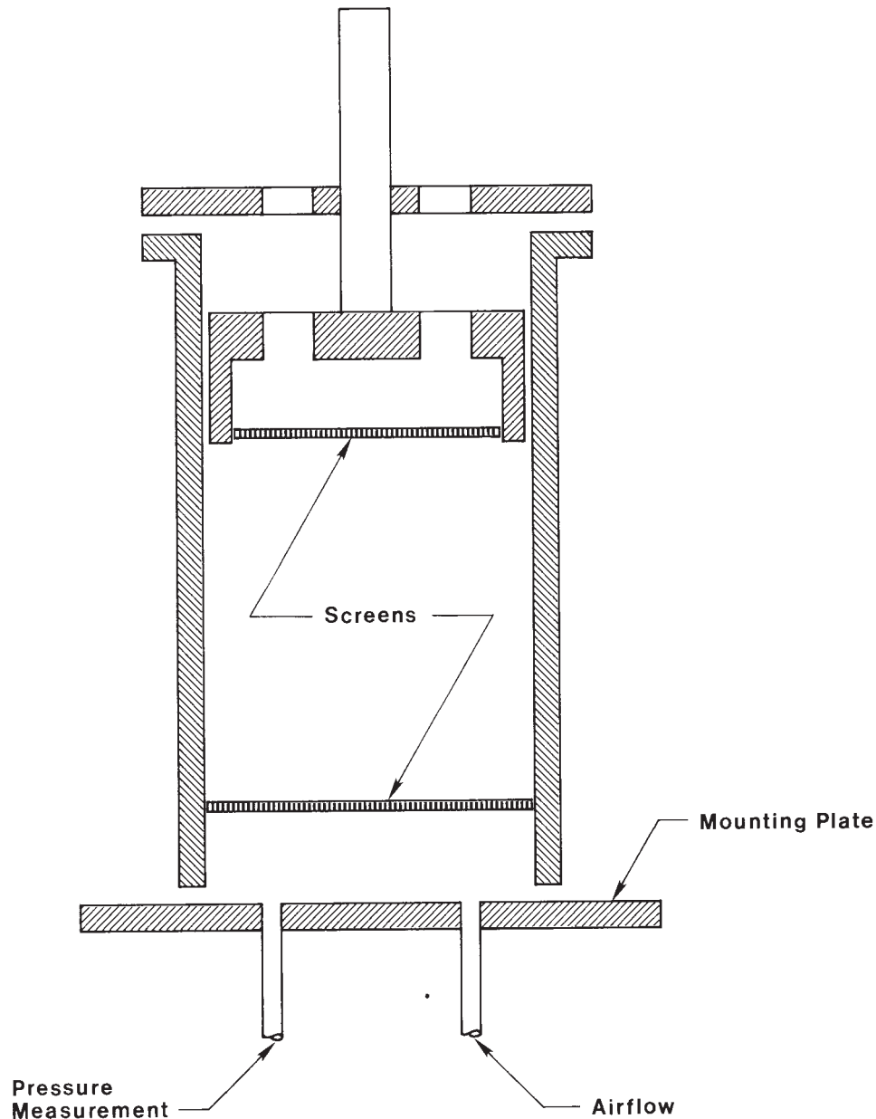
FIG. 2 Specimen Holder
