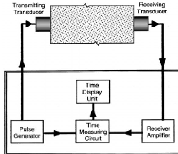
FIG. 1 Schematic of Pulse Velocity Apparatus
