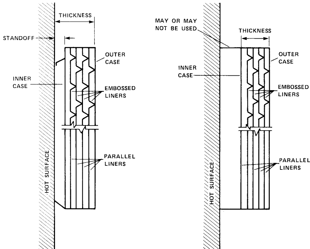
(a) Reflective Insulation Applied to Piping
