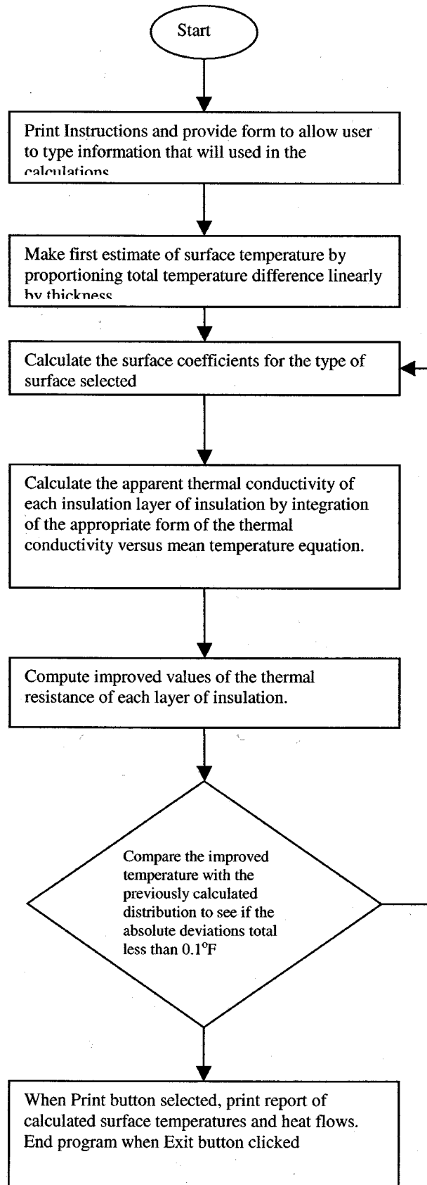
FIG. 1 Flow Chart
