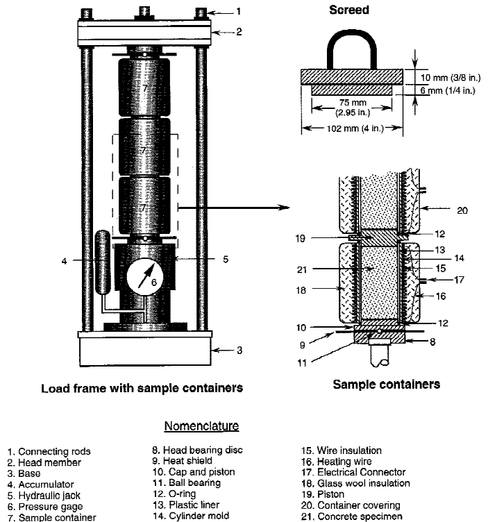
FIG. X1.3 Schematic of High-Temperature and Pressure Curing Apparatus (Procedure D)
