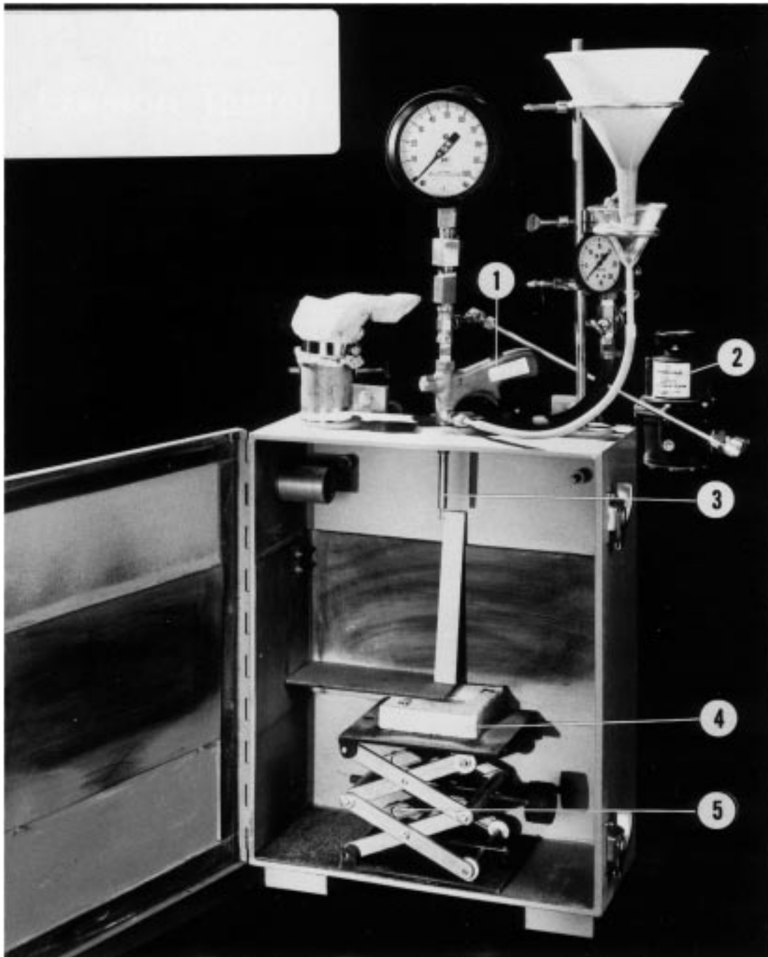
FIG. 2 Abrasion Tester
