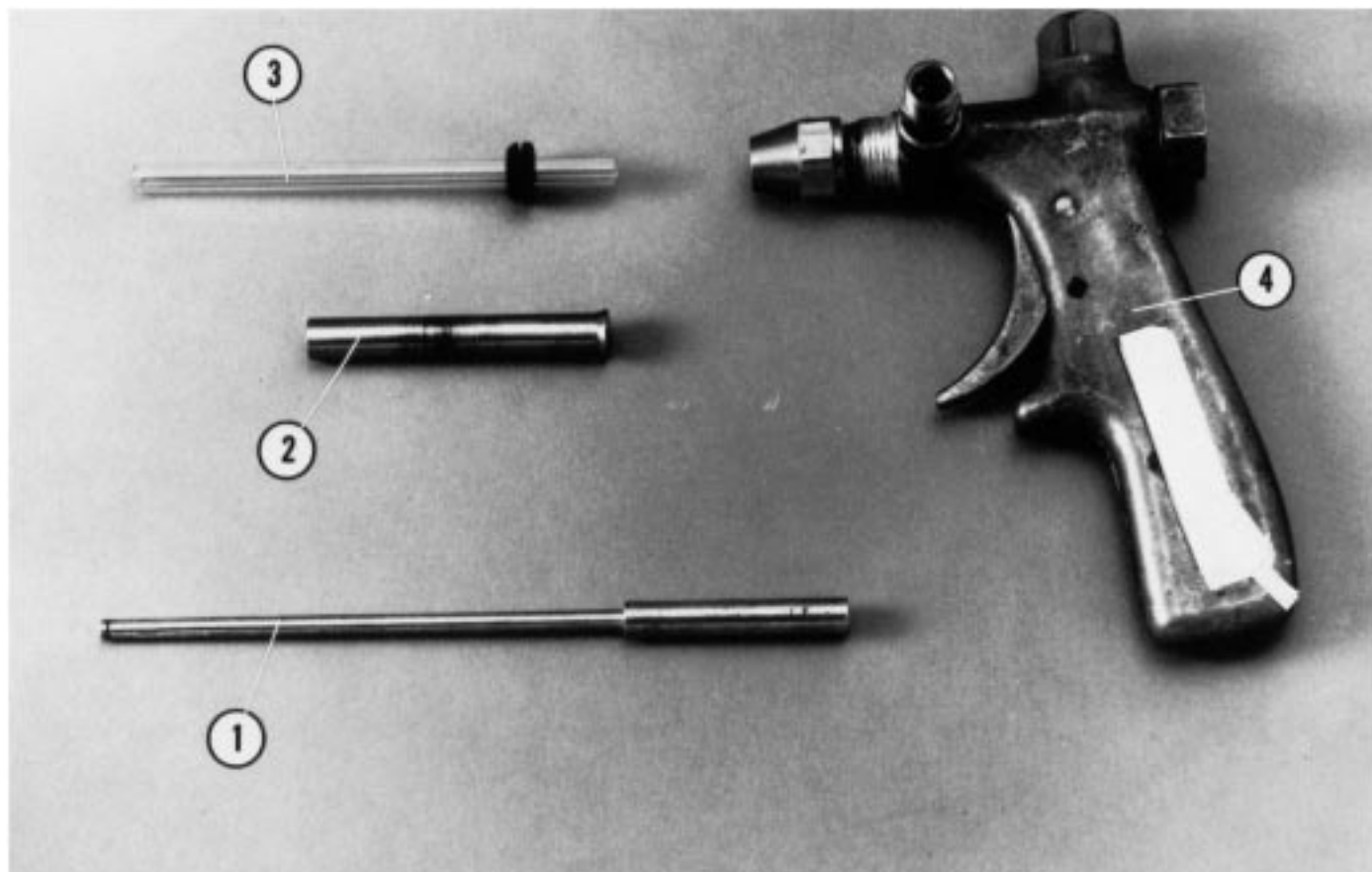
FIG. 3 Modified Blast Gun Breakdown
