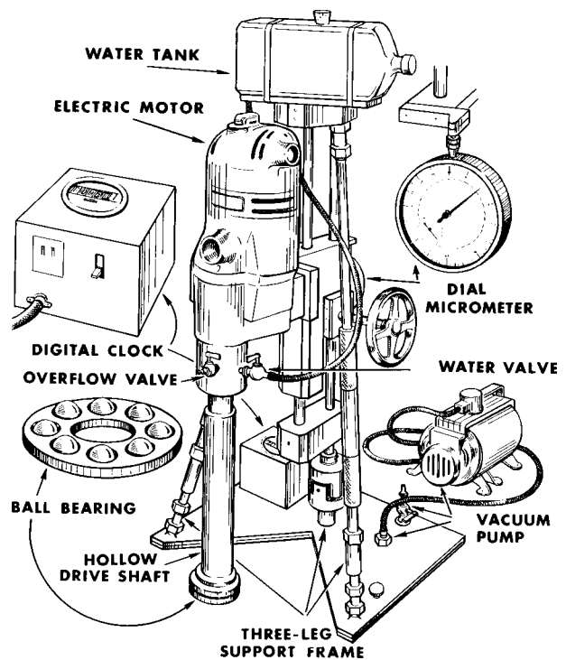
FIG. 3 Ball Bearing Abrasion Test Machine
