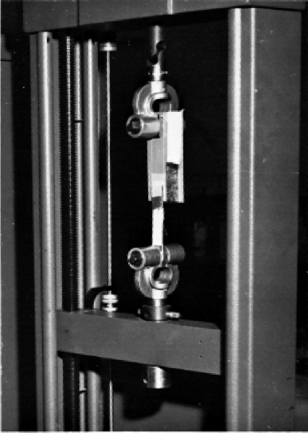
FIG. 2 Extension Machine Used in the Adhesion-in-Peel Test
