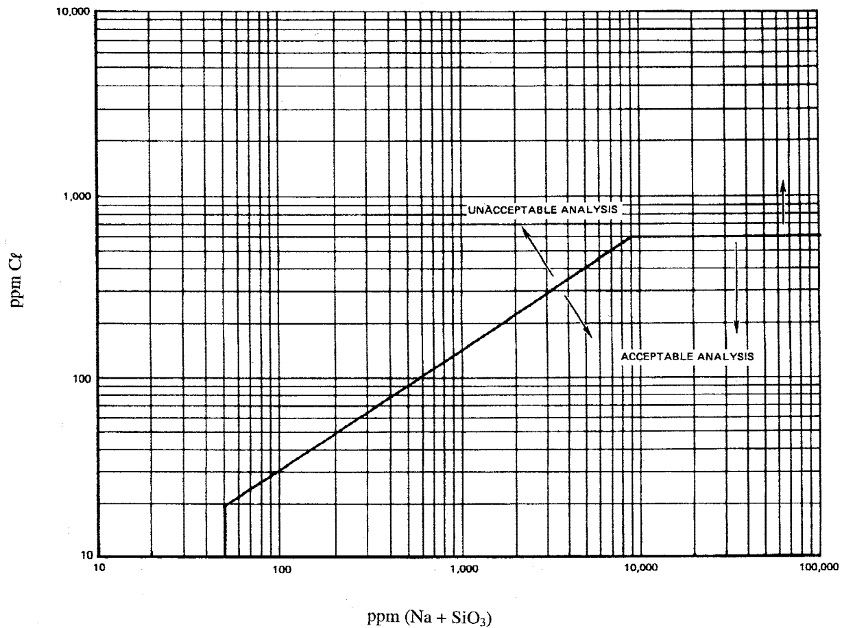
FIG. 1 Acceptability of Insulation Material on the Basis of the Plot Points of the Cl and the (Na + SiO 3 ) Analyses.
