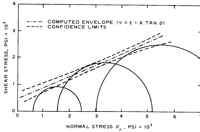
FIG. 5 Mohr's Diagram (1)
