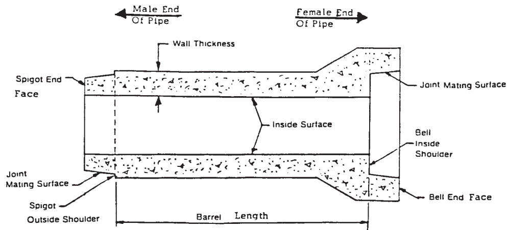
Bell and Spigot Pipe
