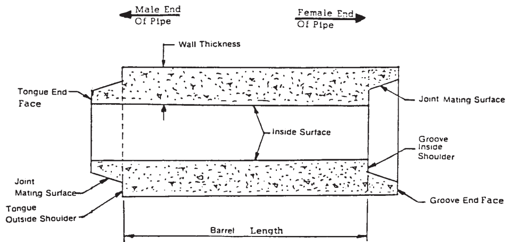
Tongue and Groove Pipe
