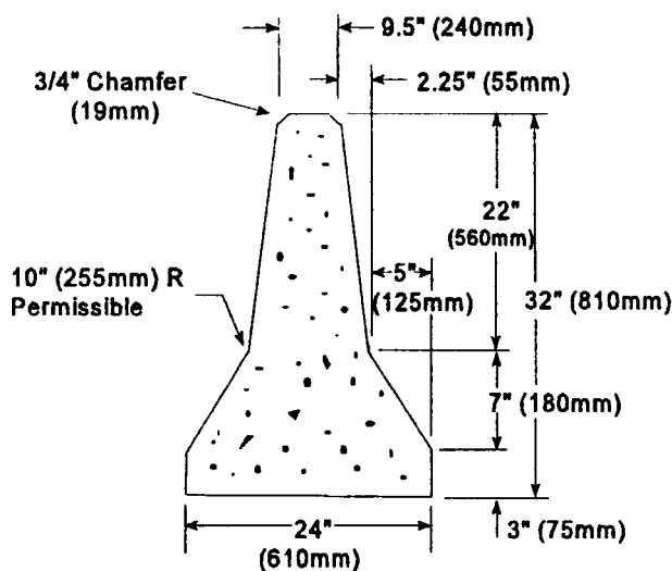
FIG. 2 Type-F Barrier
