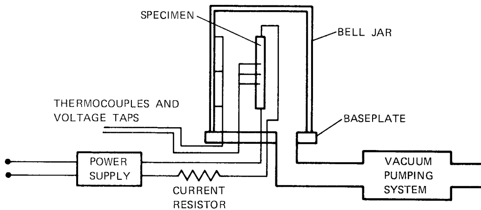
FIG. 1 System Arrangement
