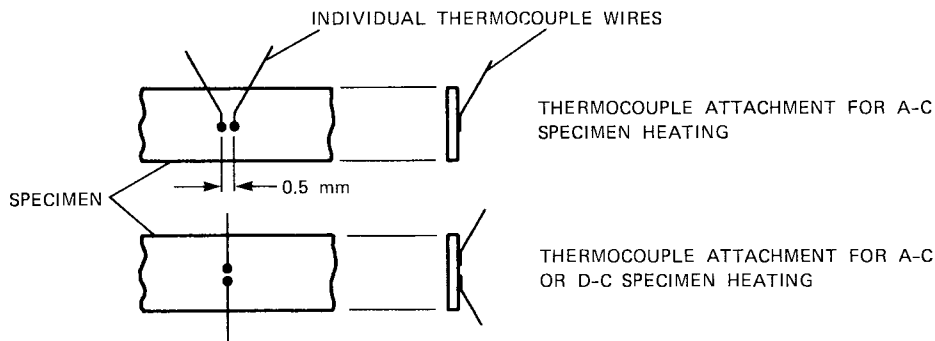
FIG. 6 Thermocouple Attachment
