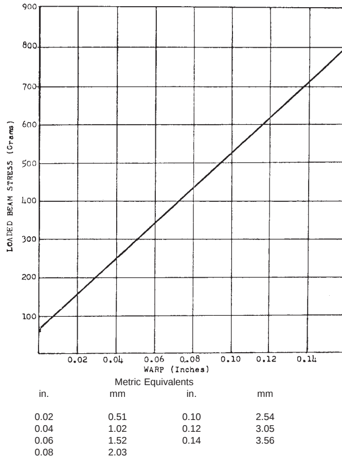
FIG. 1 Conversion Chart for Loaded-Beam Stress to Warp Stress
