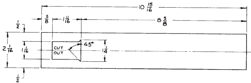
FIG. 4 Loaded-Beam Test Apparatus
