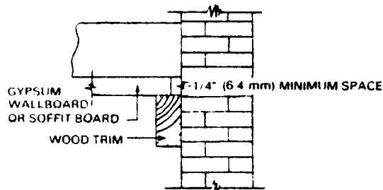
FIG. 9 Masonry Wall
