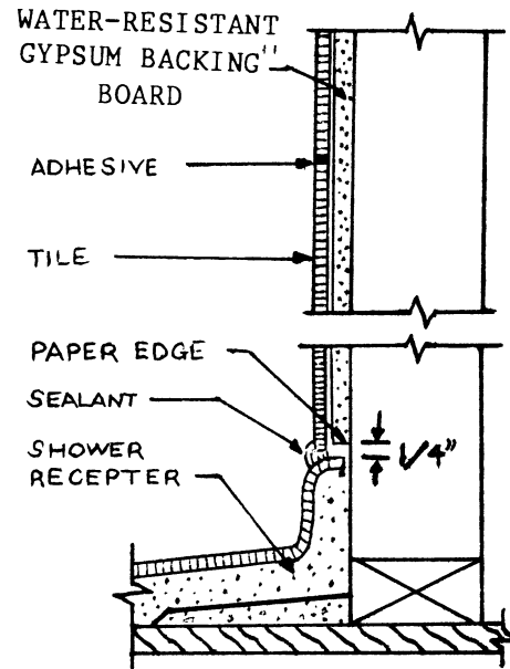
FIG. 6 Adhesive Application of Gypsum Board at Shower Where WR Board Will Receive Ceramic Tile or Other Protective Covering
