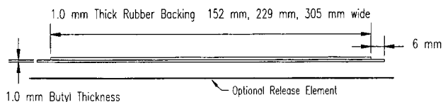
FIG. 3 Sealing Band Type III (Not to Scale)
