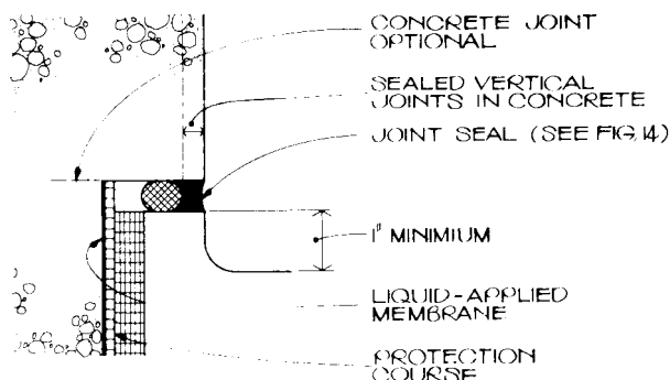
FIG. 2 Terminal Condition Above Finish Grade on Concrete Wall (see 8.3.1)
