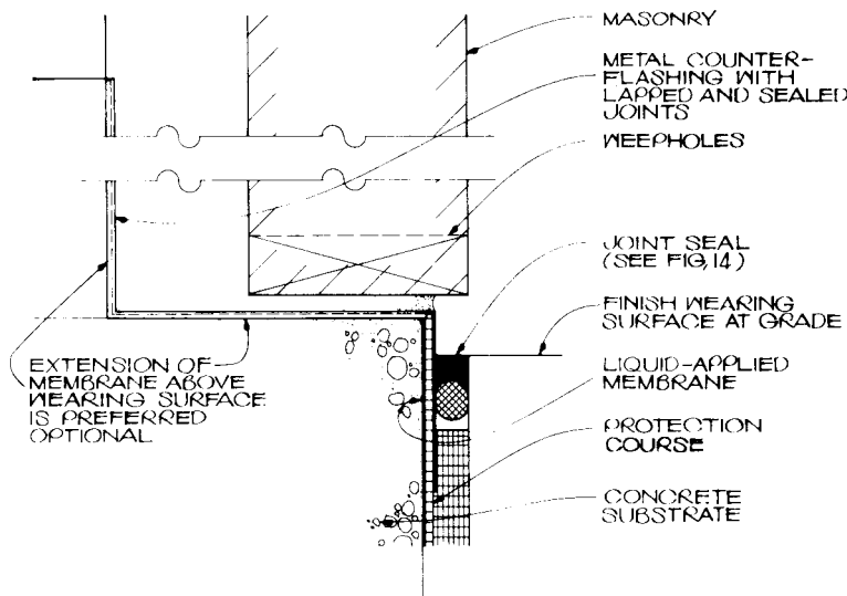
FIG. 4 Terminal Condition with Masonry Above Finish Wearing Surface at Grade (see 8.3.1)
