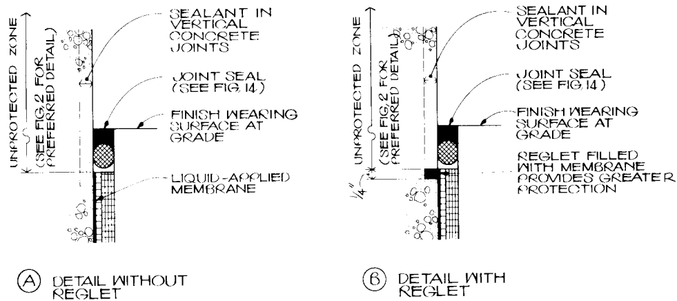
FIG. 3 Terminal Conditions on Concrete Wall Below Finish Wearing Surface at Grade (see 8.3.1)
