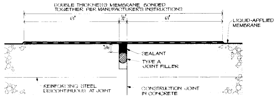
FIG. 8 Treatment of Nonreinforced Butted-Joint in Concrete Slab (see 8.4.2)
