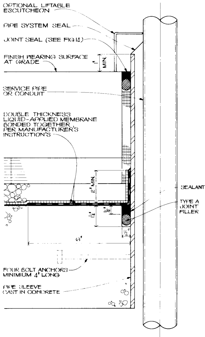
FIG. 6 Termination at Pipe Penetrations (see 8.3.3 and 18.9)
