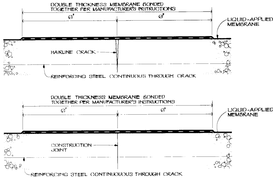
FIG. 7 Treatment of Reinforced Cracks and Joints in Concrete Slab (see 8.4.1)
