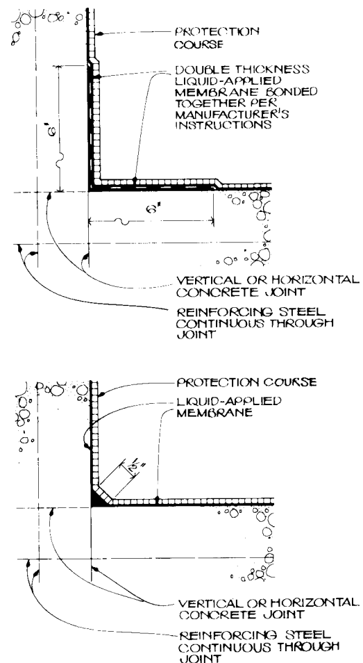
FIG. 14 Turnup Details at Reinforced Joint (see 18.6)
