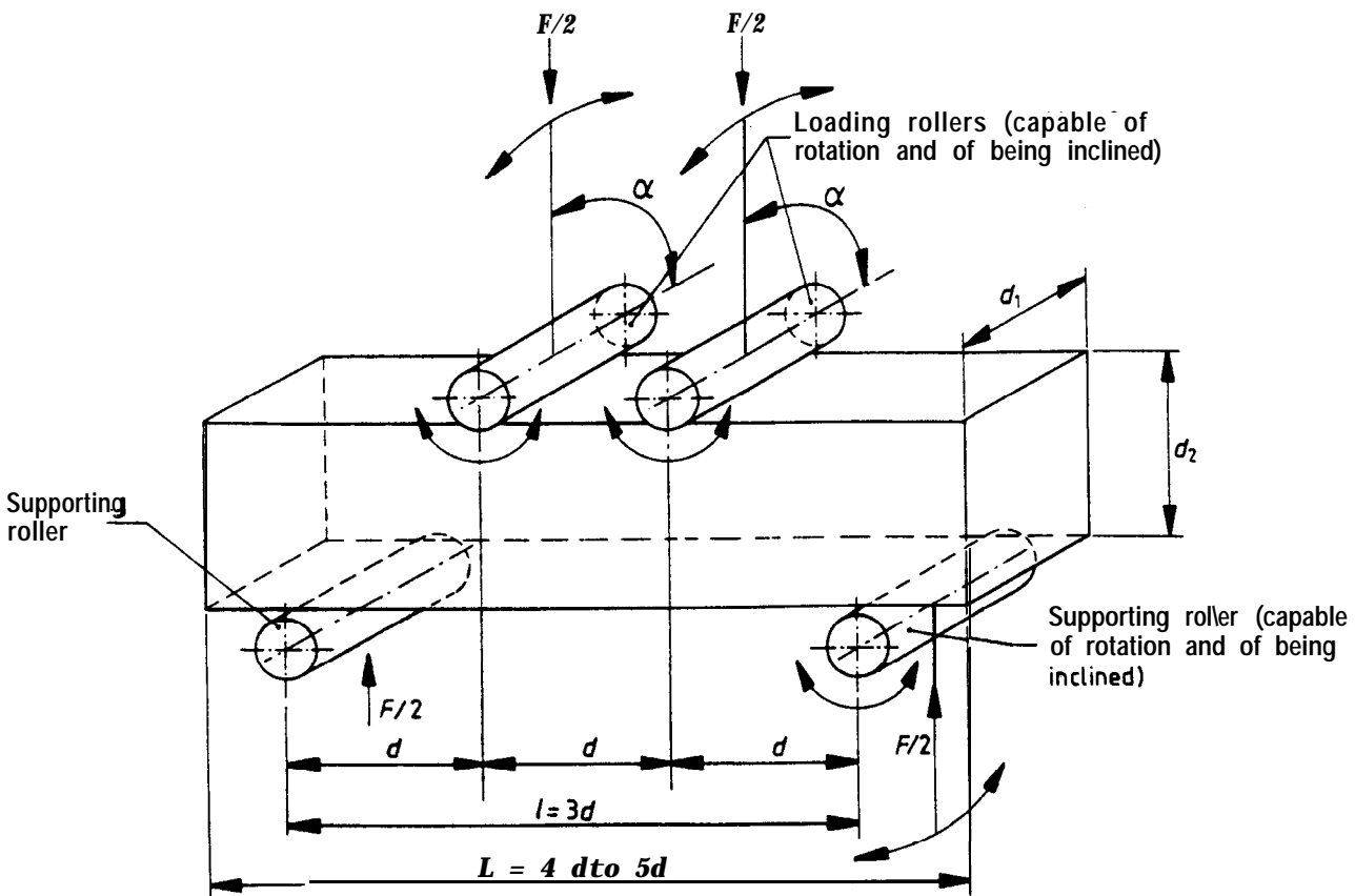
d = nominal cross-section dimension of the beam d_1, d_2 = actual dimensions.
