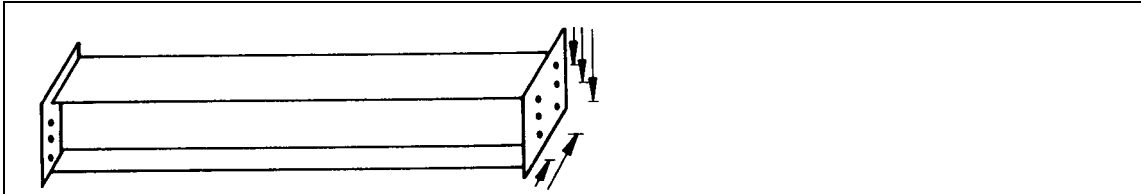
(3) position of centres of bolt holes within welded end plates [Table 2 (T.2.3)]
