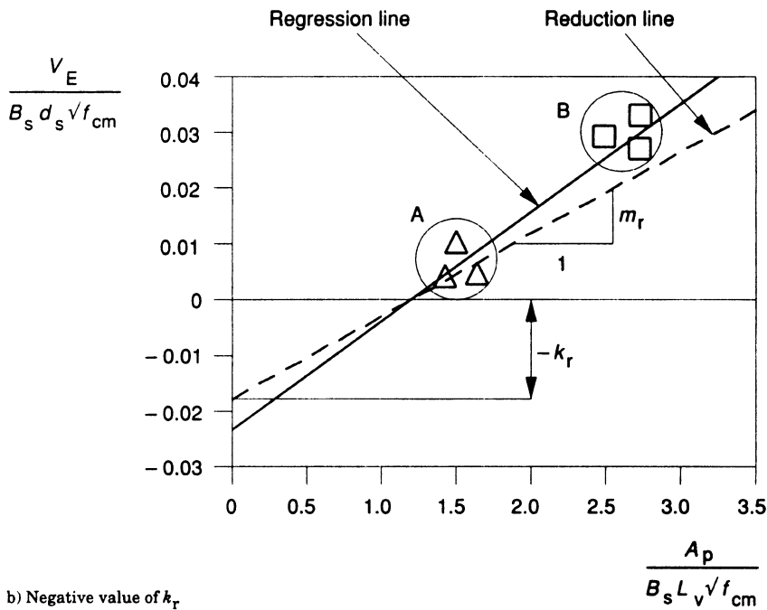
b) Negative value of k_r
