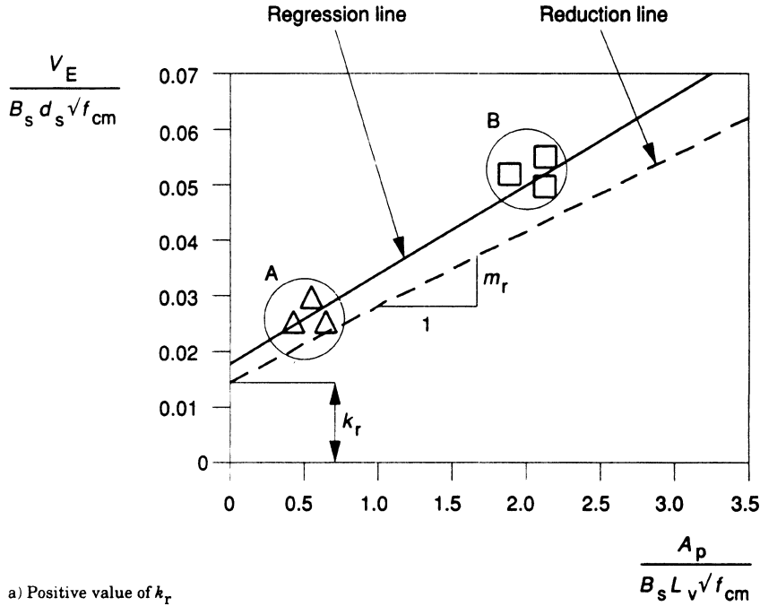
a) Positive value of k_r
