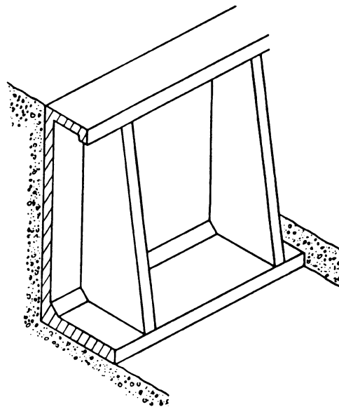
b) Reinforced concrete wall with buttresses
