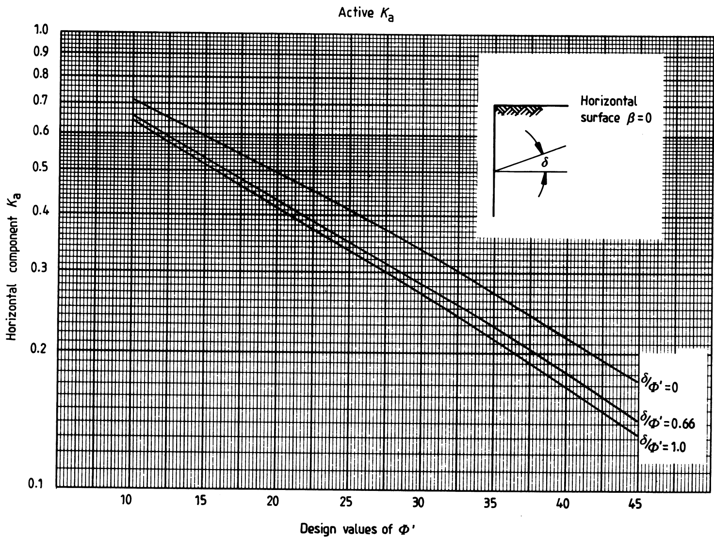
Figure A.1 — Active pressure — Horizontal ground surface behind wall: Values of K_a (horizontal component)
