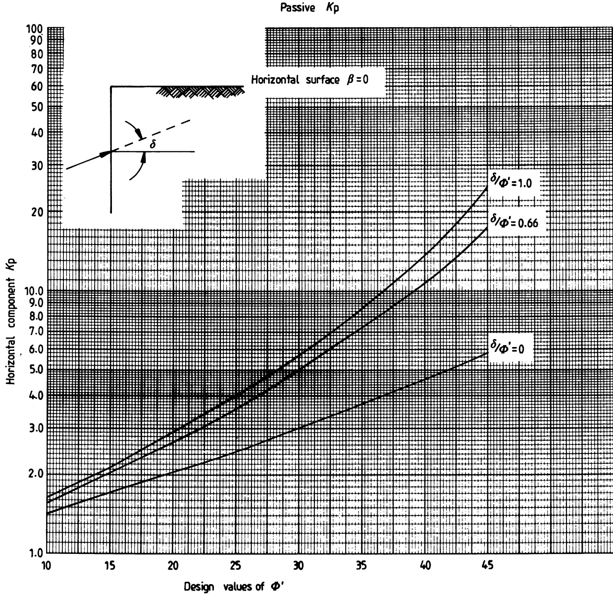
Figure A.2 — Passive resistance — Horizontal ground surface behind wall: Values of K_p (horizontal component)
