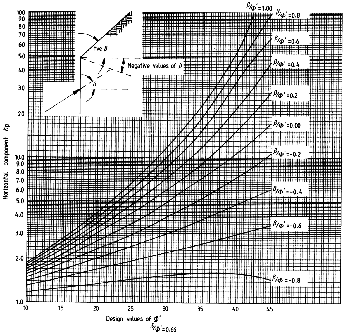
Figure A.7 — Passive resistance — Sloping ground surface behind wall: Values of K_p (horizontal component)
